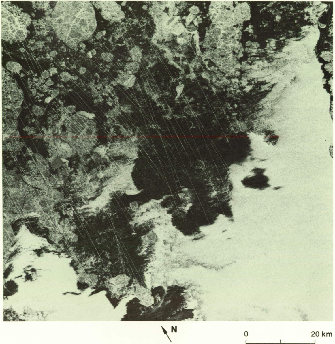
Figure 2. Seasat SAR image of the marginal ice zone off Banks Island (upper right) showing floes, grease ice (dark areas), and open water (bright areas). The image has been digitally processed and registered to an earth-based coordinate system with an accuracy of \pm 200 m. The overlain vectors, derived by JPL staff and Image Processing Laboratory software, track commonly identified floes from this image to another image (not shown) and measure the relative floe velocity over a 3-day period; Rev. 1382, October 1, 1978.
